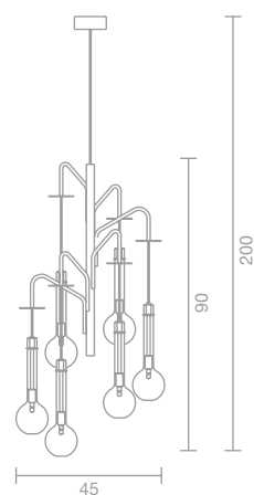
ART. 2807 Sospensione / Suspension Ø 45 h 90 h max 200 cm 6 x G9
