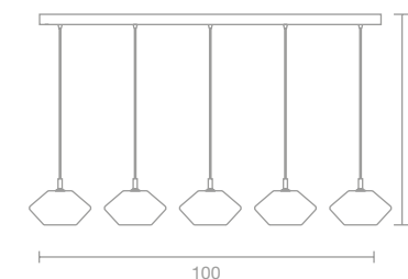
ART. 2830/5L Sospensione / Suspension L 100 h max 200 cm 5 x G9
