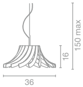
ART. 1053 Sospensione /Suspension Ø 36 h max 150 cm 1 x E27
