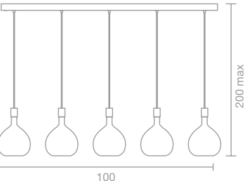
ART. 2850/5L Sospensione /Suspension L 100 h max 200 cm 5 x G9 Kg. CE IP 4,05 20
