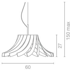
ART. 1054 Sospensione /Suspension Ø 60 h max 150 cm 1 x E27
