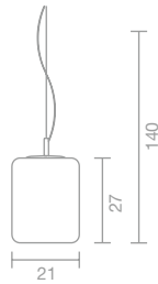
ART. 2771 Sospensione /Suspension Ø 21 h 27 h max 140 cm 1 x E27
