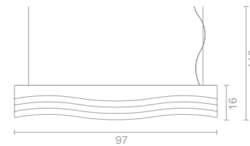
ART. 1106LED Sospensione /Suspension 97 x 16,5 h 16 h max 110 cm 40W STRIP LED
