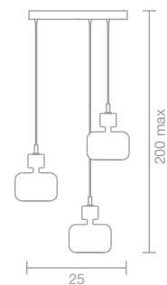
ART. 2820/3T Sospensione /Suspension Ø 25 h max 200 cm 3 x G9
