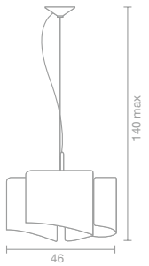
ART. 0370/3 Sospensione /Suspension Ø 46 h max 140 cm 3 x E27
