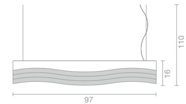
ART. 1107LED Sospensione vetro /Glass suspension 97 x 16,5 h 16 cm h max 110 cm 40W STRIP LED
