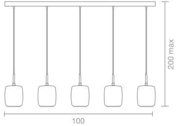
ART. 2840/5L Sospensione / Suspension L 100 h max 200 cm 5 x G9
