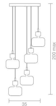
ART. 2820/5T Sospensione /Suspension Ø 35 h max 200 cm 5 x G9
