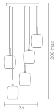
ART. 2840/5T Sospensione / Suspension Ø 35 h max 200 cm 5 x G9
