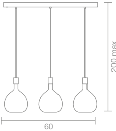
ART. 2850/3L Sospensione /Suspension L 60 h max 200 cm 3 x G9 Kg. CE IP 2,6 20
