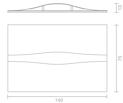
ART. 4501 Applique /Wall lamp 140 x 75 h 13 cm R7s LED
